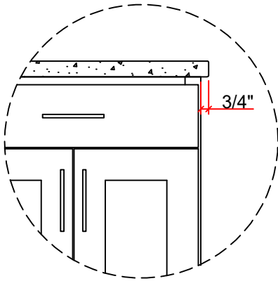
KITCHEN 3/4" OVERHANG AT OPEN ENDS
