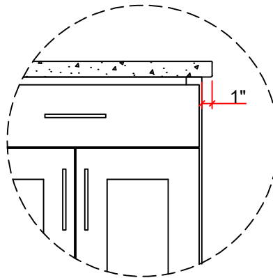
VANITY 1" OVERHANG AT OPEN ENDS
