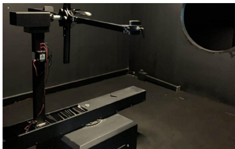
GMP-Goniophotometer
