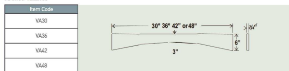
Arched Valance
